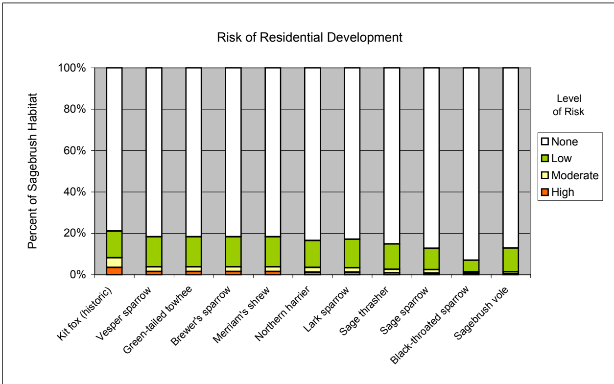
Figure 6-14. Percentage of sagebrush habitat at risk for each species of concern of residential development and energy development.
