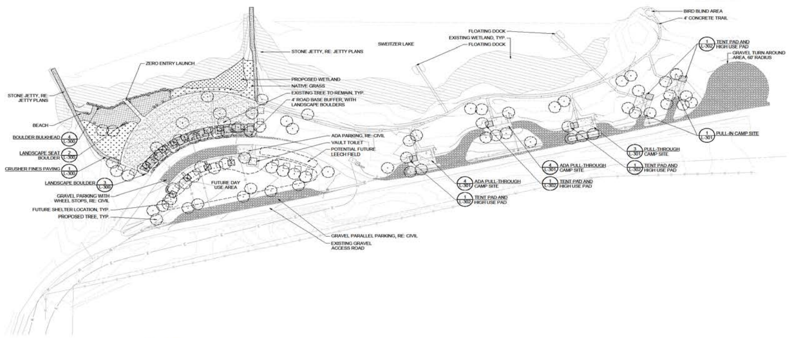
1 OVERALL LANDSCAPE PLAN
