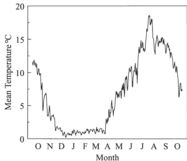
Fig. 3. Mean daily temperature (°C) at the Breeze Bridge holding site (September 16, 1997, to October 14, 1998)
