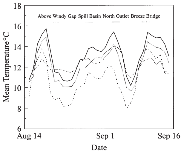
Fig. 2. Mean daily temperature (°C) at the 4 exposure locations during the exposure period (August 14 to September 16, 1997)
