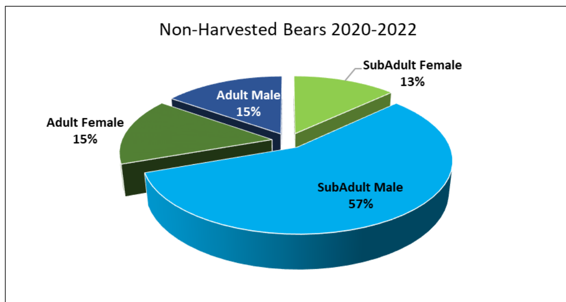
Figure 17. Age and sex composition of non-harvested bears in B-16, 2020-2022 (n=46 bears).
