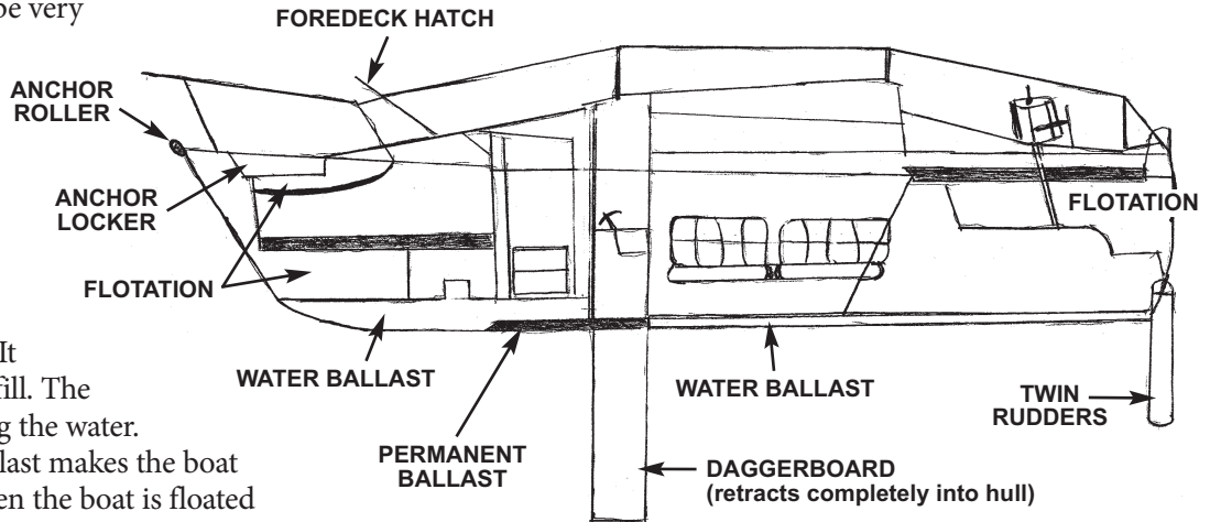
The diagram above represents a schematic of the MacGregor sailboat and its complexities.
