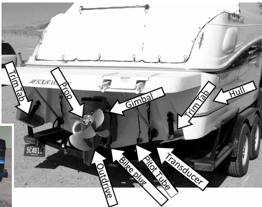
DIAGRAM © WEN BALDWIN, PSMFC ANS TRAINING CONTRACTOR
