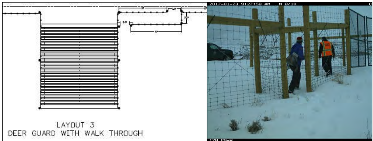
Figure 7-3. Left: CDOT design for pedestrian access point adjacent to a wildlife guard. Right: People walking through a pedestrian access point.
