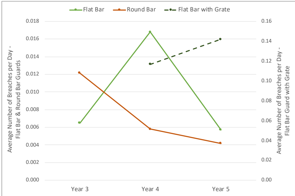
Figure 5-4. Average number of breaches per monitoring day by guard type Years 3-5. During this timeframe, six flat bar guards were monitored, five round bar guards, and one flat bar guard with a pedestrian grate.
