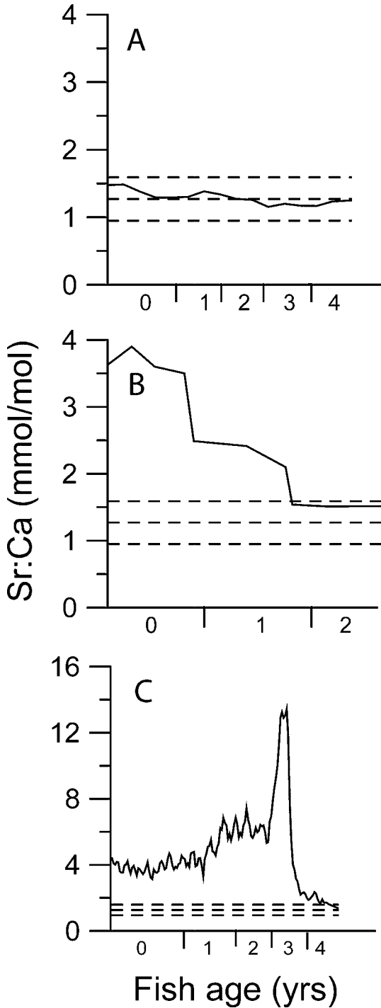
FIGURE 2.—Representative patterns of otolith strontium:calcium ratios (Sr:Ca) along laser-ablated transects from the core to the edge of the otolith for individual fish collected from the Colorado River and its backwaters. Data are shown for (A) an age-4 green sunfish, (B) an age-2 green sunfish, and
