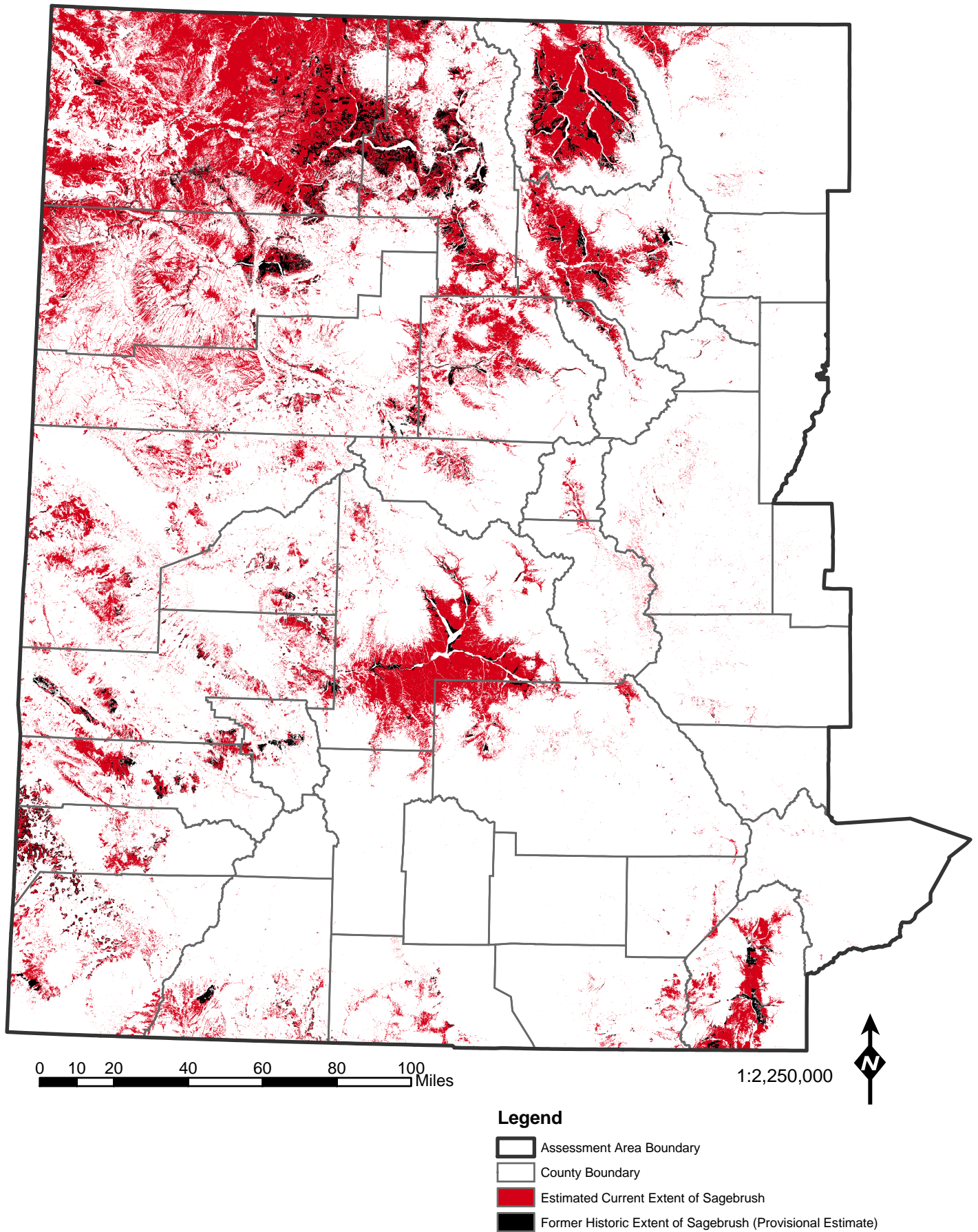
Figure 3-1. Current and historic sagebrush distribution in the assessment area.
