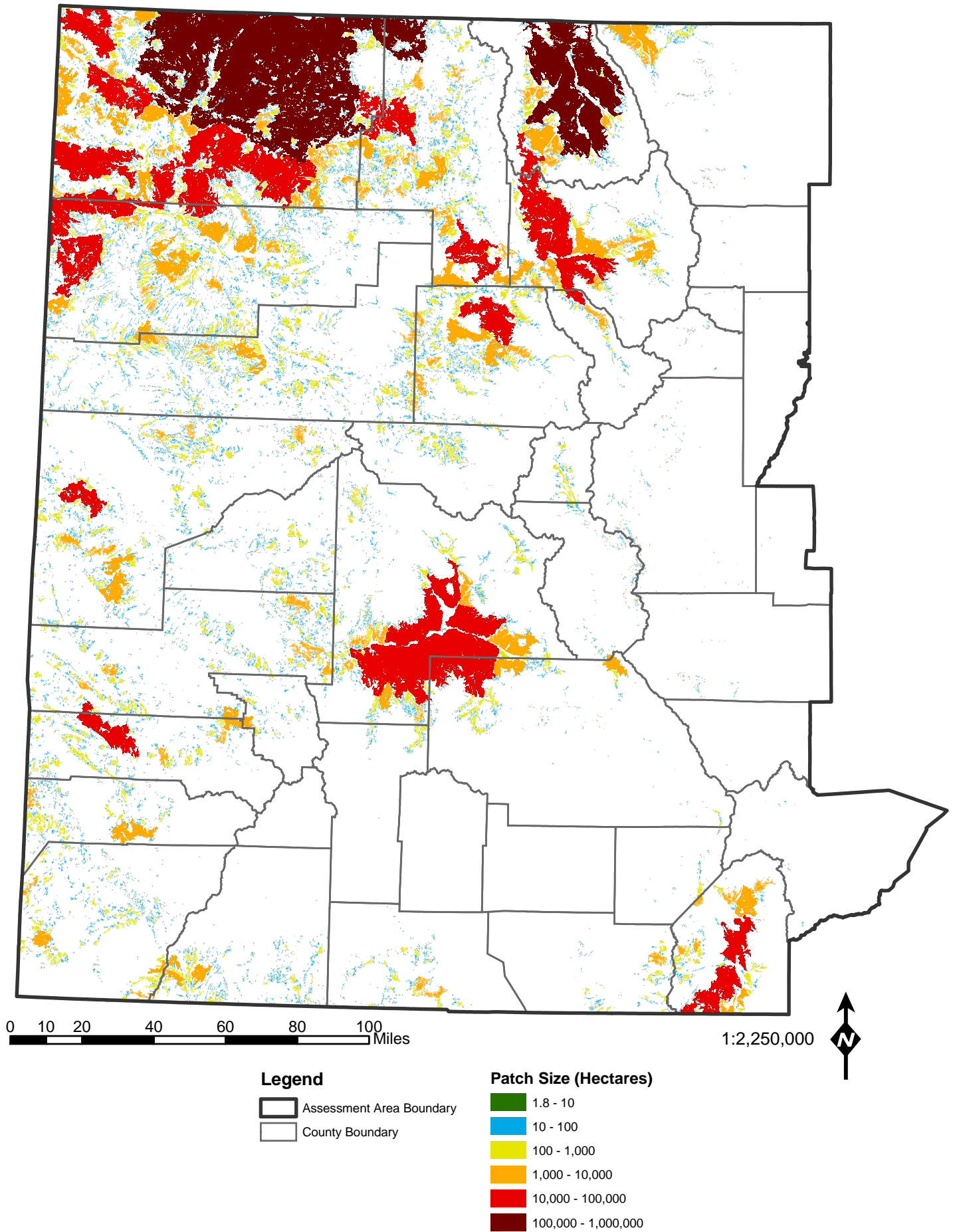
Figure 3-3. Current sagebrush patch size distribution.
