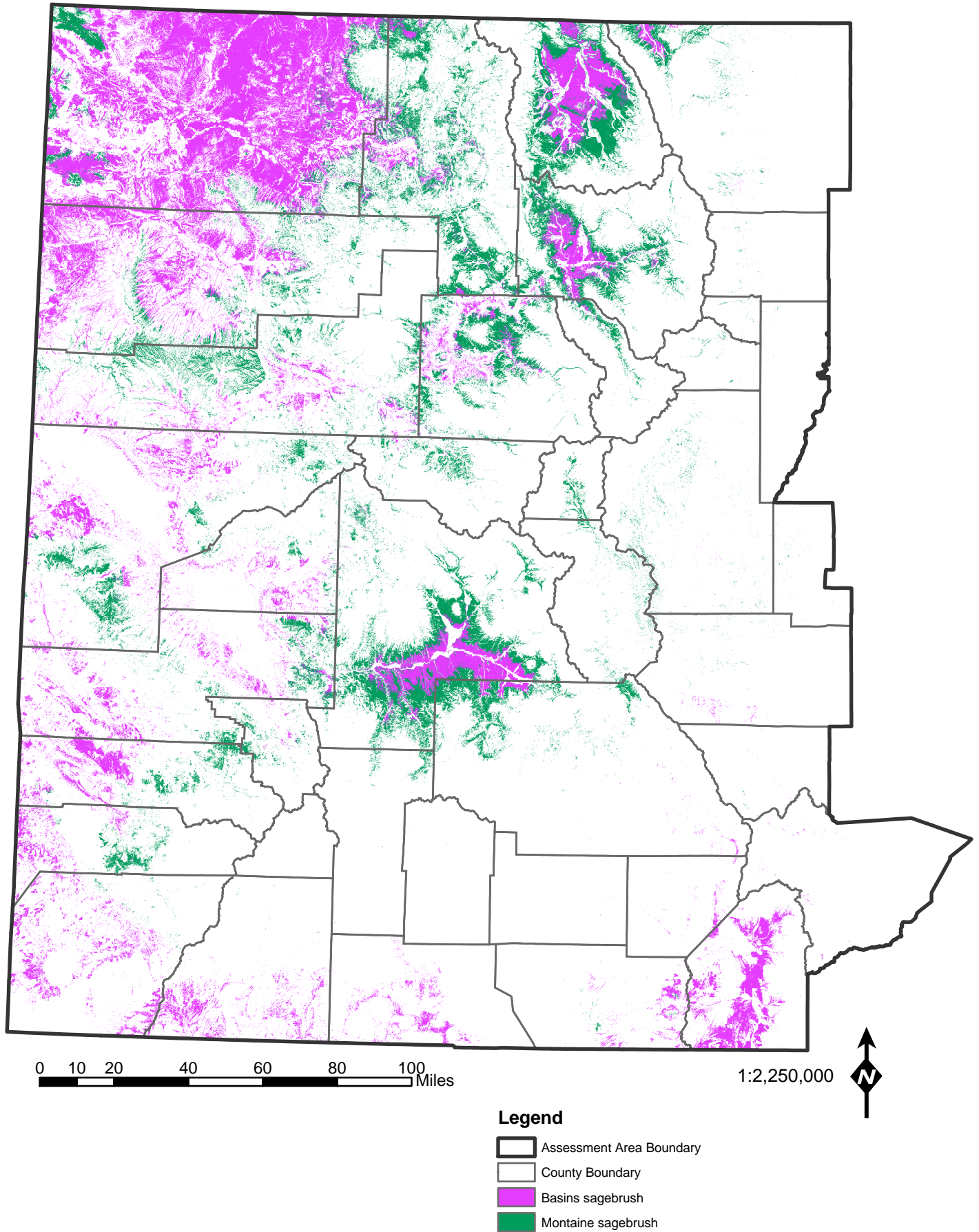
Figure 3-4. Current distribution of montane and basins sagebrush in the assessment area.
