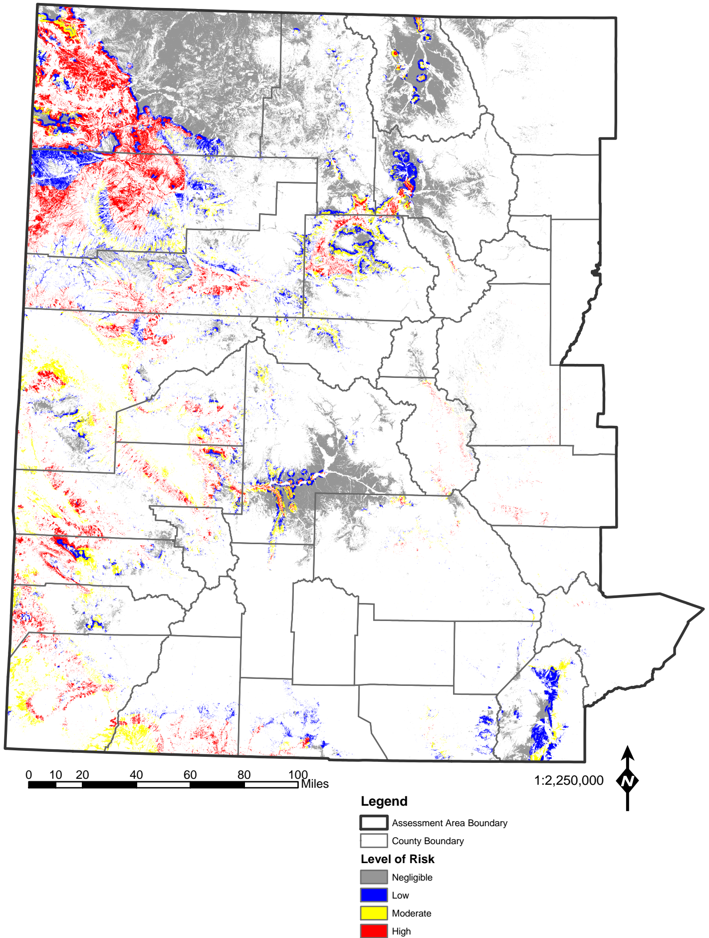
Figure 4-1. Sagebrush at risk from pinyon-juniper encroachment.
