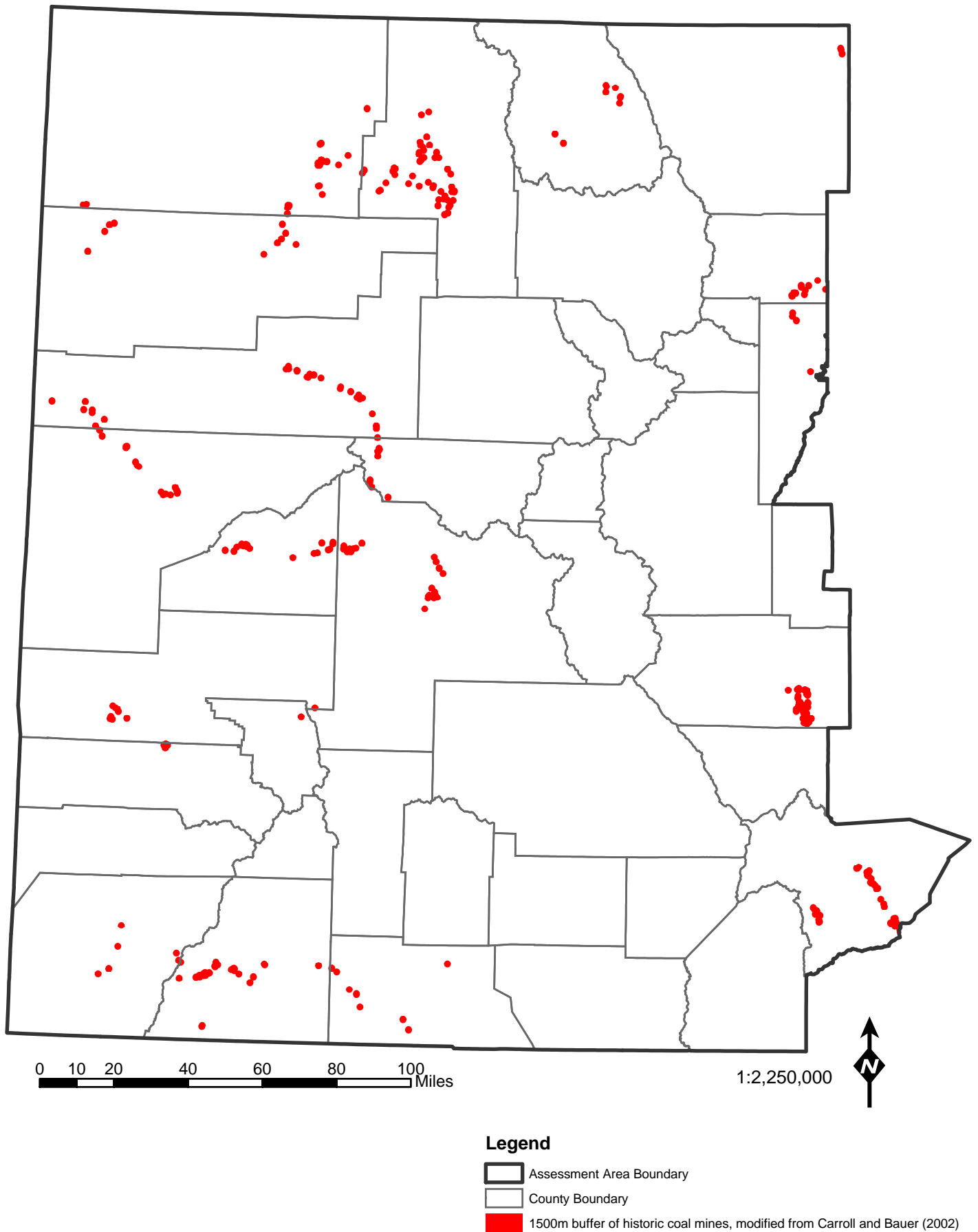
Figure 4-11. 1,500 meter buffer of historic coal mines in the assessment area, modified from Carroll and Bauer (2002).
