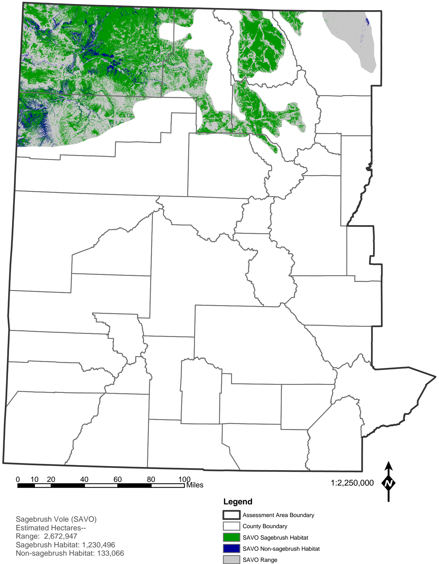
Figure 6-10. Sagebrush vole range and habitat.
